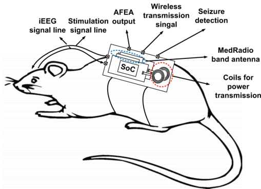
Fig. 2. The measurement setup of the microsystem with SoC on a freely-moving Long-Evans rat.
